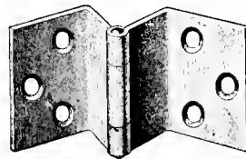
Fig. 2608. POCKET-HINGE.
